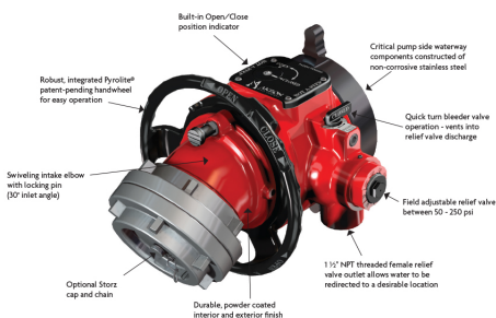
Revolution intake valve diagram
