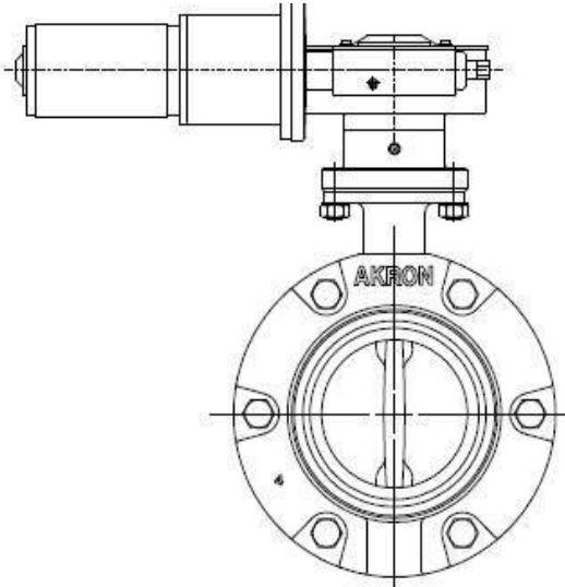
Electric actuator
