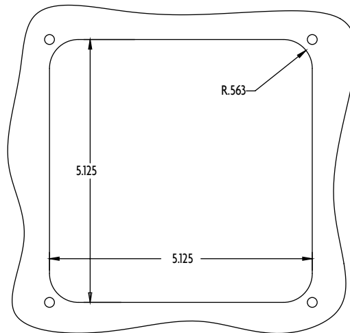
RECCOMENDED OPENING FOR FLUSH MOUNTING (TO SCALE)
