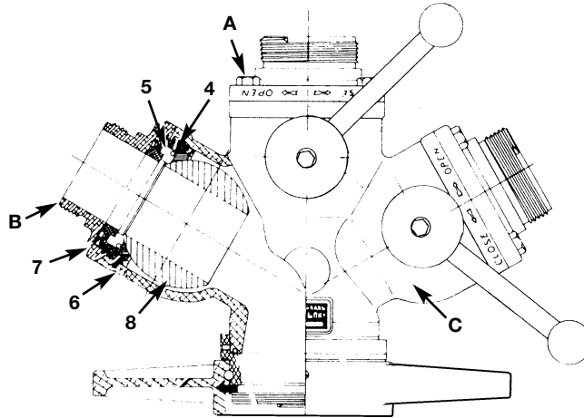
STYLE 1573 2 1/2" VALVE ONLY
