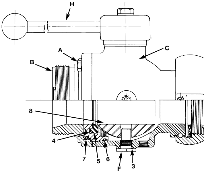
STYLE 828 2 1/2" VALVE
