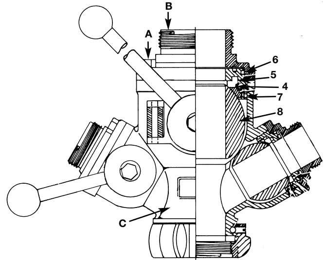
STYLE 1573 2 1/2" VALVE ONLY
