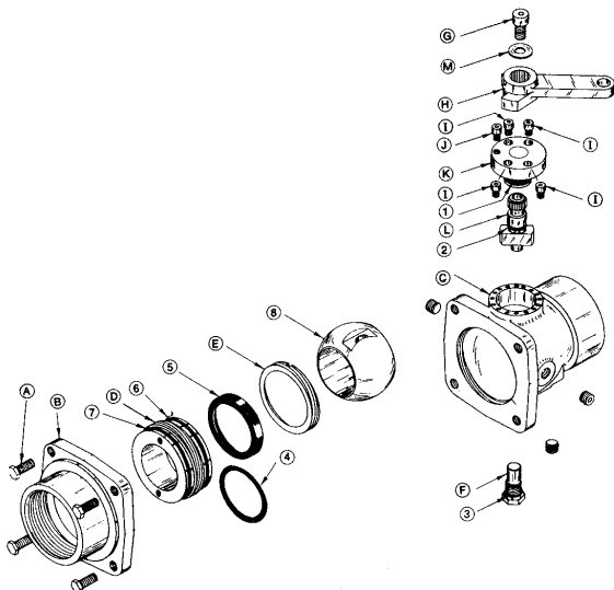
STYLE 828 2 1/2" VALVE
